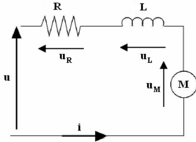
Figure 2.1: Electrical scheme of a DC motor
