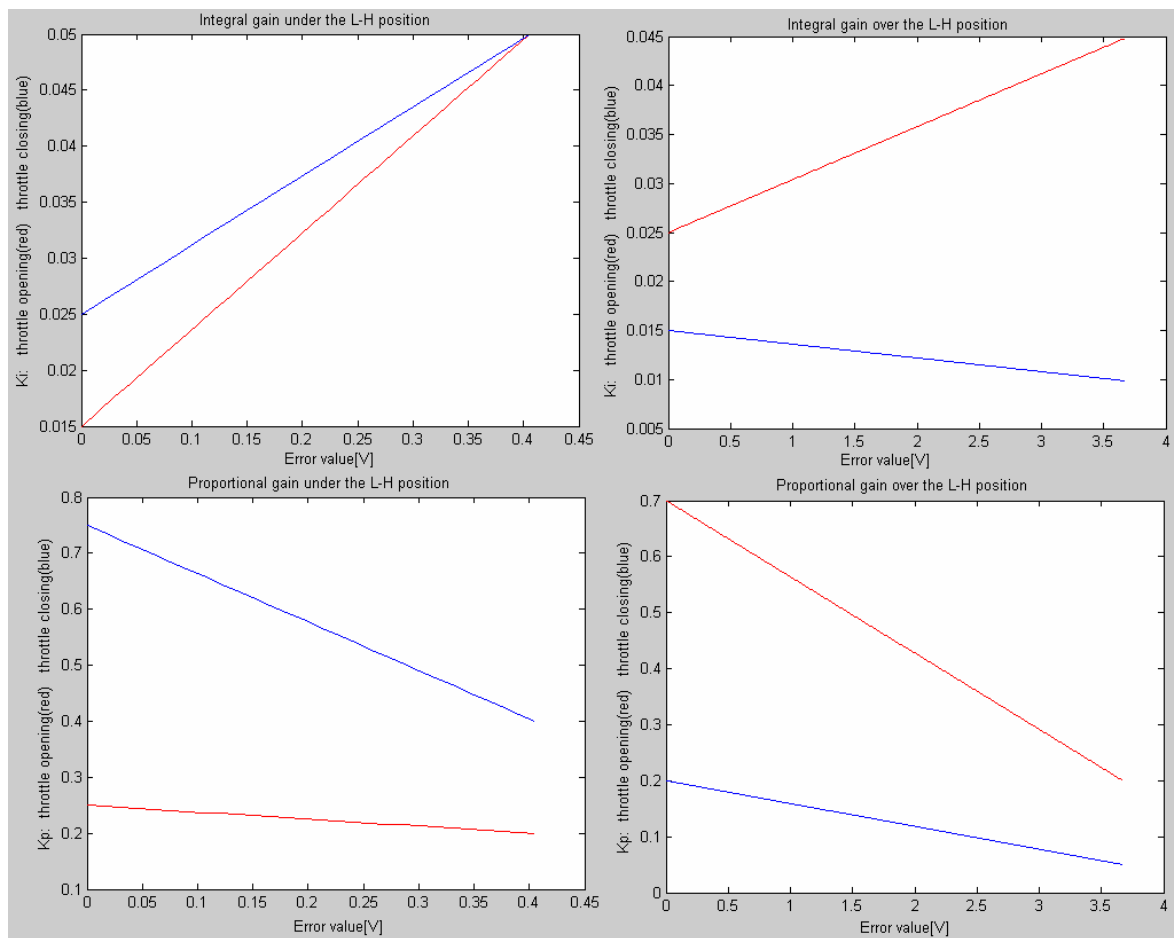
Figure 4.4: K_p and K_i parameters under and over LH position
