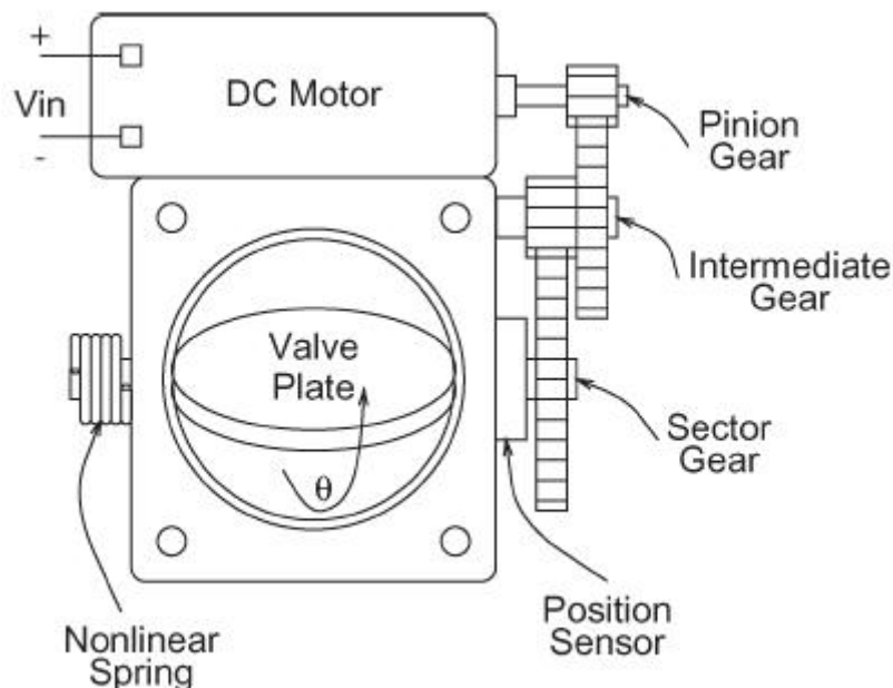
Figure 1.1: Electronic Throttle Body
