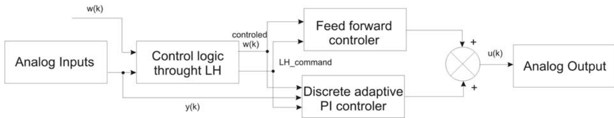
Figure 4.1: Structure of the control system
