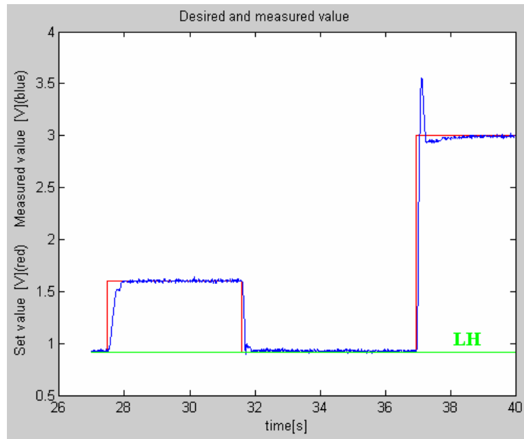
Figure 4.3: Closed-loop step response with discrete PI with constant parameters K_p , K_i .
