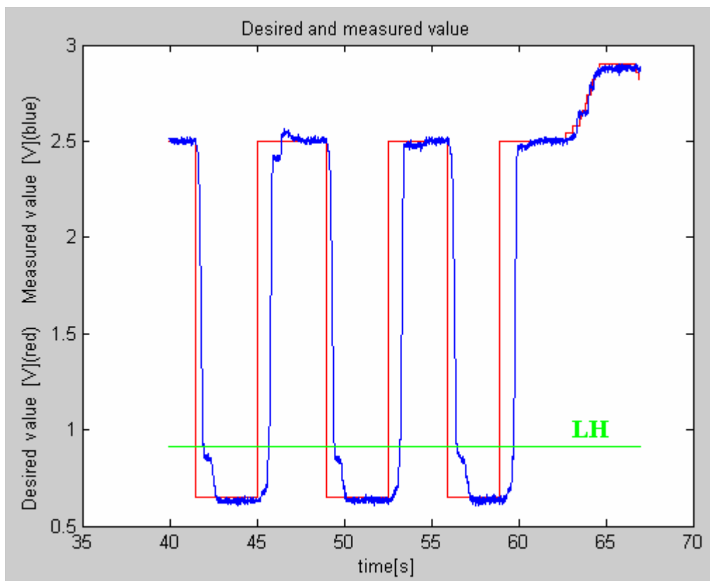
Figure 4.5: Closed-loop step response with discrete PI with scheduled parameters K_p , K_i
